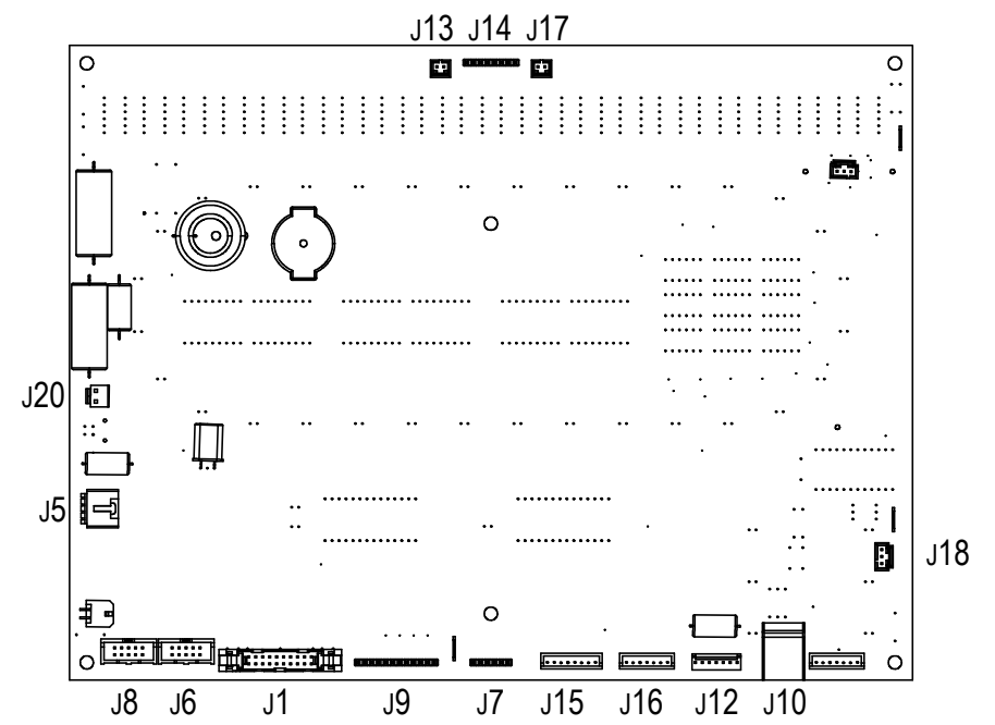
CONNECTOR DESIGNATIONS ON PCB Ⓢ P/N 715-3845
